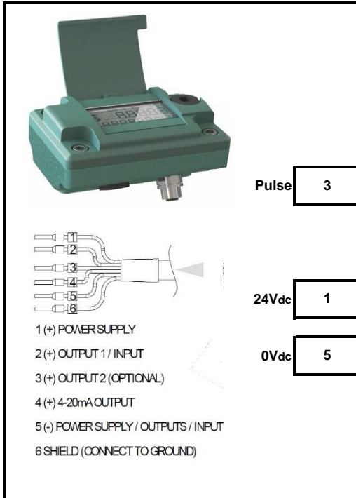
MV800 flow converter
