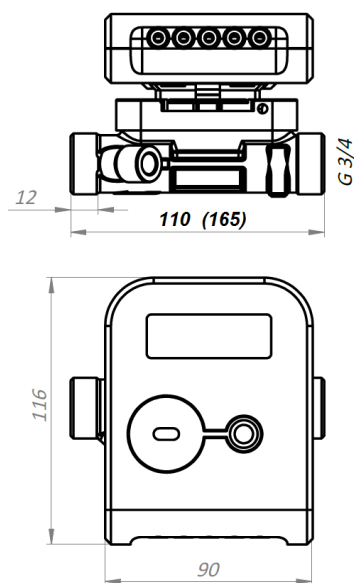
Fig. B2.1 Flow sensor q_p = 0.6/1.0/1.5 \text{ m}^3/\text{h} Length L = 110 \text{ mm} ( L = 165 \text{ mm} ); connection type: thread G 3/4"
