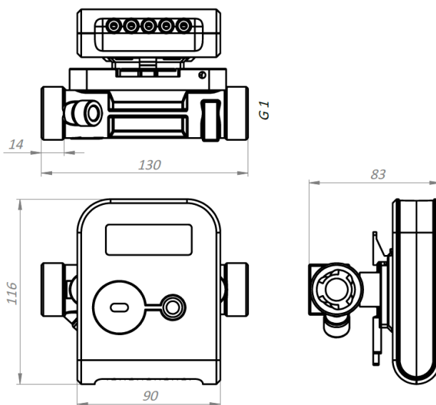
Fig. B2.2 Flow sensor q_p = 2.5/1.5 \text{ m}^3/\text{h} Length L = 130 \text{ mm} ; connection type: thread G 1"
