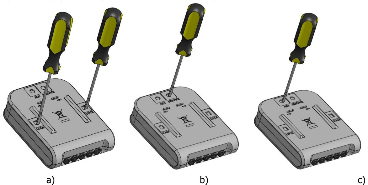
Fig. 4.1 Access to elements fixing the opening of the box (a), configuration change activation contacts, and adjustment data change activation contacts (c) (partitions easily breakable with a tool)
